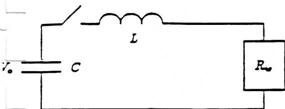
Figure 1: Water Arc Discharge Circuit
